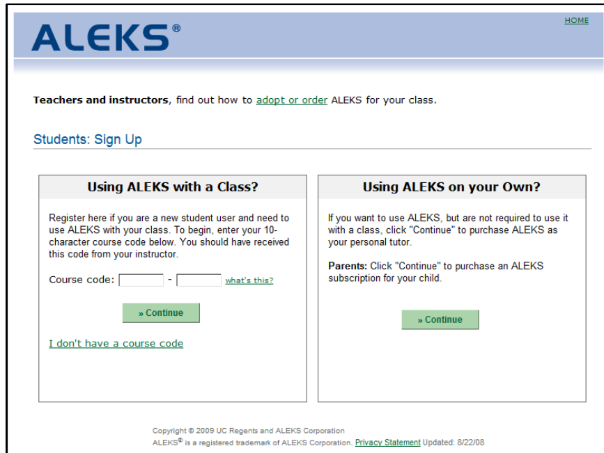
Figure 2: Course Code
