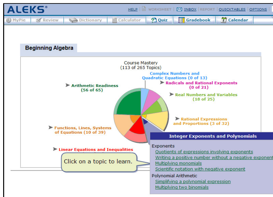
Figure 5: Assessment Report
